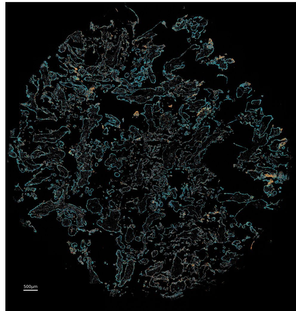
slidetags_with_permissiveness W8-2
